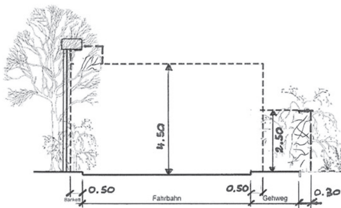
--- Lichtraumprofil
